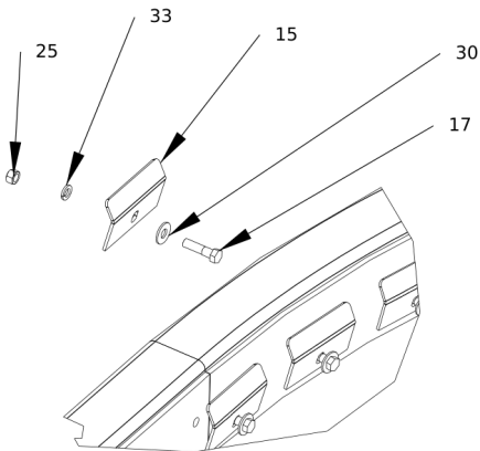
DETAIL C SCALE 1/8
