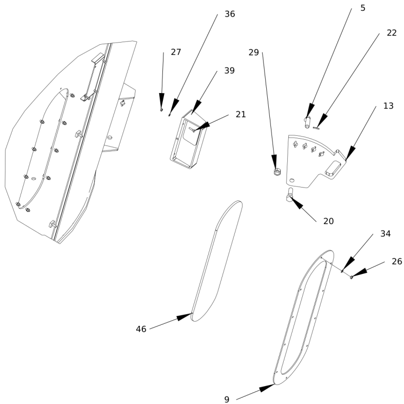
DETAIL A SCALE 1/16
