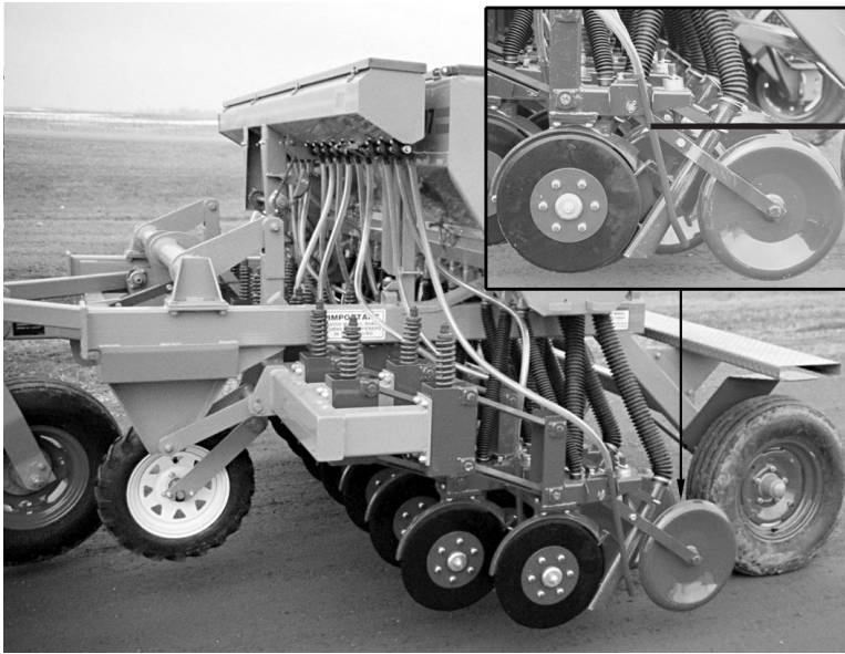
drop tube with seed tube connected
