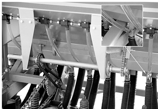
Completed drive shaft and seed tubes shown with standard hose connections. (See following page for completed drive shaft with optional drop tube assembly installed.)
